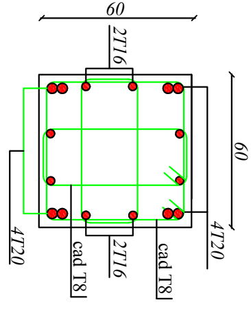
zone1:Poteau(60x60)
