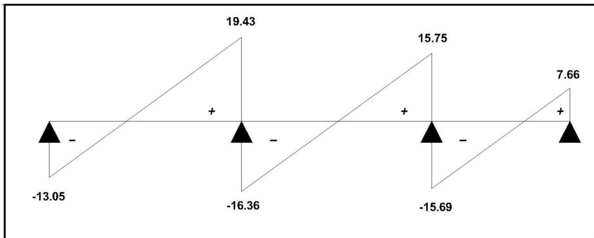
Figure III.12: Diagramme des efforts tranchants "Poutrelle terrasse inaccessible".
