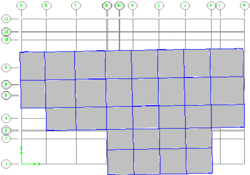
Figure IV.3: Mode 2 (Translation x-x).
