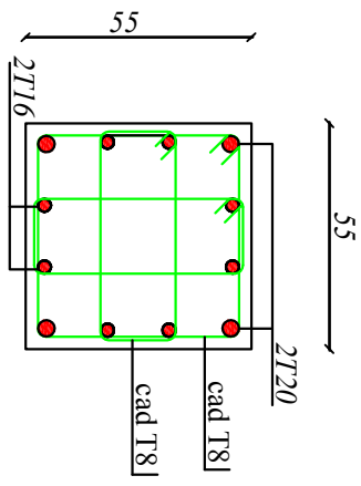
zone2:Poteau(55x55)
